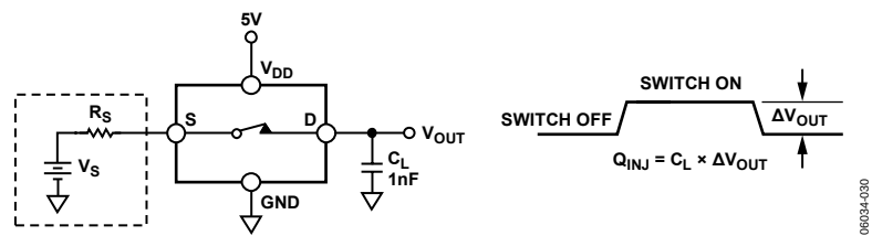
Figure 30. Charge Injection
