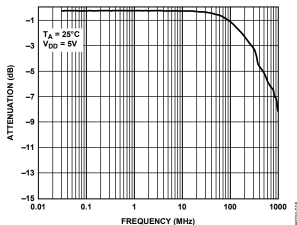
Figure 15. Bandwidth
