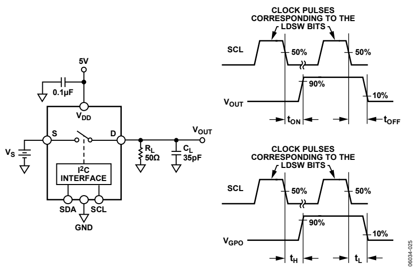
Figure 28. Switching Times
